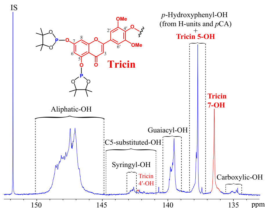
Fig. 7. ^{31}\text{P} NMR spectrum of tritordeum straw MWL phosphitylated with TMDP and using NHND as an internal standard (IS) for quantification.
